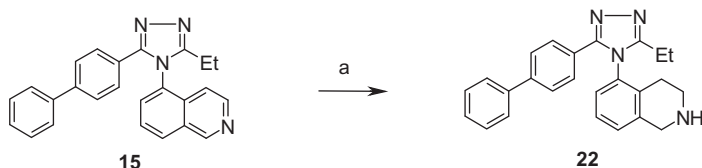
Scheme 5. Reagents: (a) NaBH 3 CN, AcOH.
