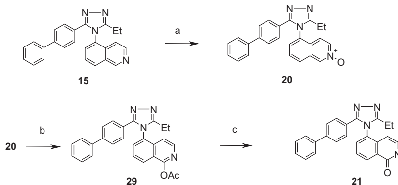
Scheme 4. Reagents and conditions: (a) m CPBA, CH 2 Cl 2 ; (b) Ac 2 O, 120 °C; (c) NaOH, MeOH.
