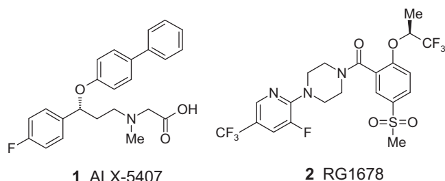
Figure 1. Structures of ALX-5407 ( 1 ) and RG1678 ( 2 ).
