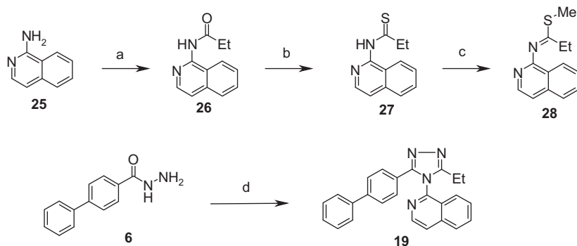
Scheme 3. Reagents and conditions: (a) EtCOCl, pyridine, THF; (b) Lawesson's reagent, pyridine, 100 °C; (c) MeI, NaOH, EtOH; (d) 28 , p -TsOH-H 2 O, xylene, 130 °C.
