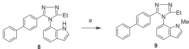
Scheme 2. Reagents: (a) MeI, KOH, DMF.
