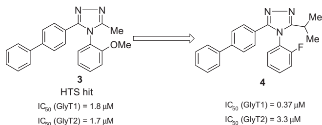
Figure 2. In our previous work, modification of HTS hit 3 led to identification of compound 4 .
