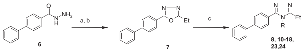
Scheme 1. Reagents and conditions: (a) EtCOCl, Et 3 N, DMF; (b) POCl 3 , 100 °C, (c) R-NH 2 , p -TsOH-H 2 O, 160–200 °C.
